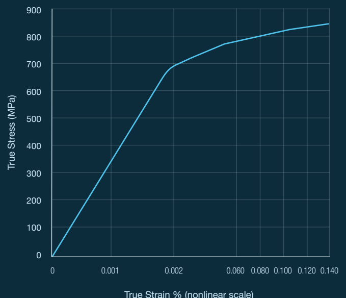
UltraTube™ Non-linear stress strain curve (typical)
